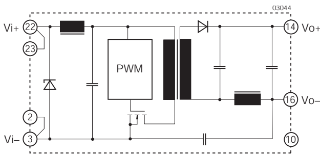
Fig. 1 Block diagram for single-output models with standard pinout.
