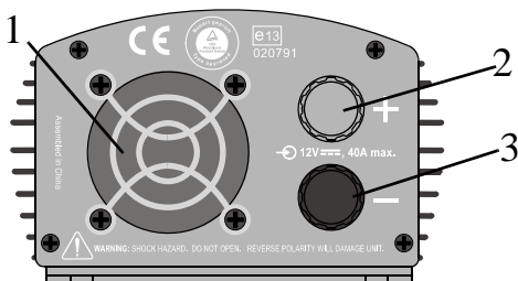
Figure 5 DC Panel on the XPower 300
